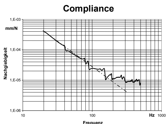
Compliance Curve for a type HDT Optical Tabletop (Size 1200x1800x300mm, Point Load 114kg in middle of the table, excitation by sinus sweep 20-500Hz)
